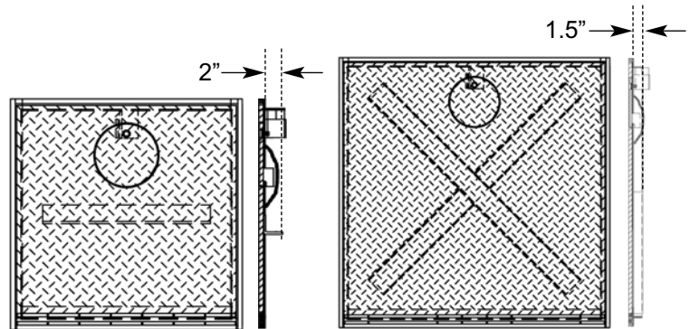
The 24" and 30" vaults are reinforced with 2"x2"x1/4" steel angle
