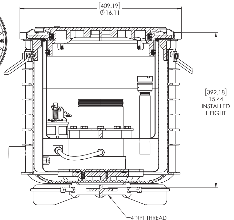
SECTION G-G SCALE 1 : 1.5
