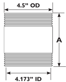
A7901: Controlled ID
