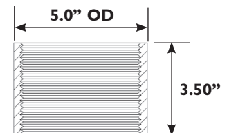
A7904-004 Merchant Steel Coupling
