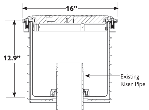
Slip-On
