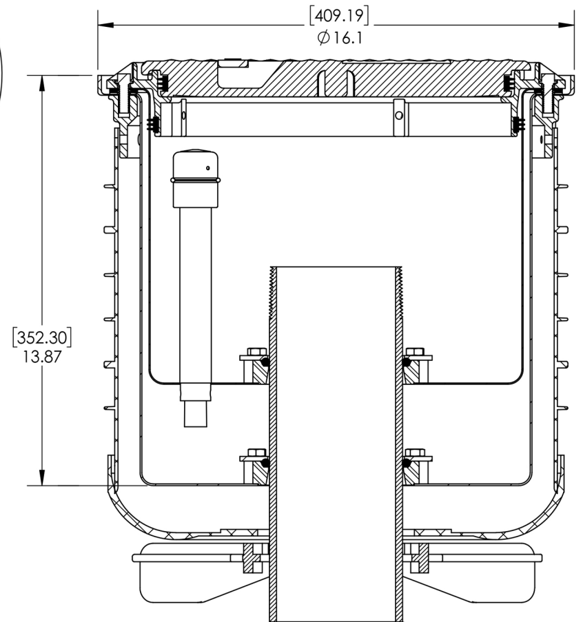
SECTION A-A SCALE 1 : 4 RISER PIPE SUPPLIED BY INSTALLER
